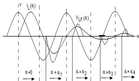
Fig. 3. Operating waveforms
