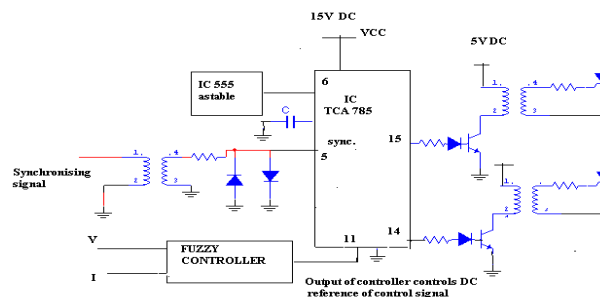
Fig.12. Firing Scheme with TCA 785 IC
